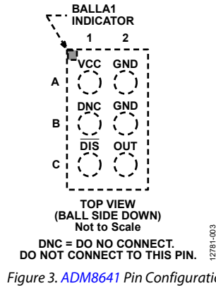
Figure 3. ADM8641 Pin Configuration
