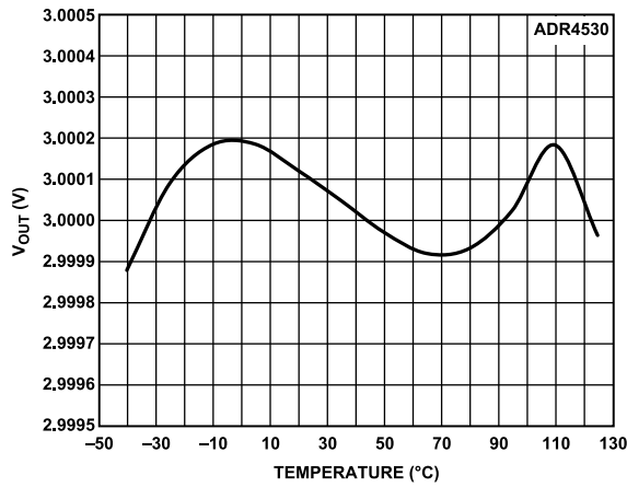
Figure 39. ADR4530 B Grade Output Voltage vs. Temperature
