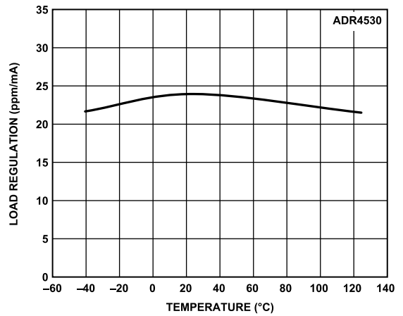
Figure 42. ADR4530 Load Regulation vs. Temperature (Sourcing)
