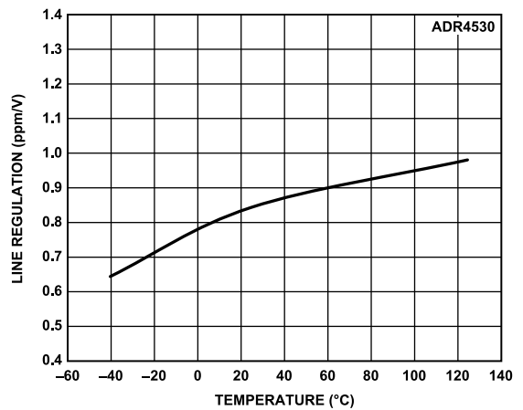
Figure 44. ADR4530 Line Regulation vs. Temperature
