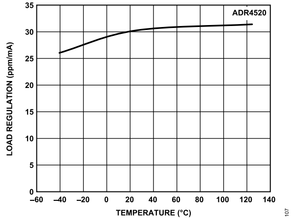
Figure 8. ADR4520 Load Regulation vs. Temperature (Sourcing)
