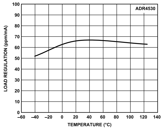
Figure 43. ADR4530 Load Regulation vs. Temperature (Sinking)
