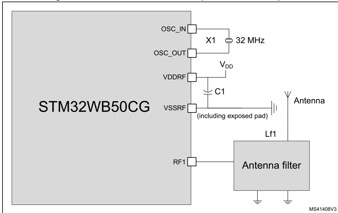
Figure 3. STM32WB50CG external components for the RF part
