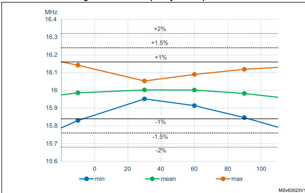
Figure 16. HSI16 frequency vs. temperature
