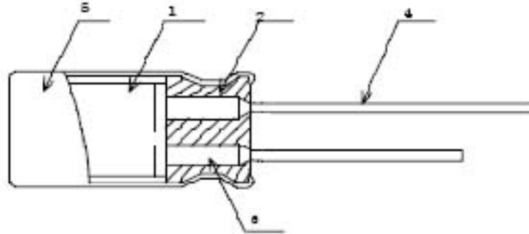
Fig. 1 Cross-section view
