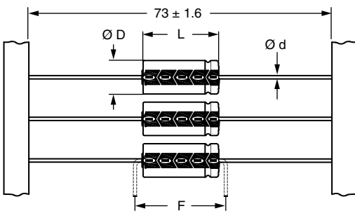
Form BA: taped in box (ammopack) Case \varnothing D \times L = 6.5 \text{ mm} \times 18 \text{ mm} to 10 \text{ mm} \times 25 \text{ mm} Form BR: taped on reel Case \varnothing D \times L = 6.5 \text{ mm} \times 18 \text{ mm} to 15 \text{ mm} \times 30 \text{ mm}
