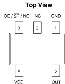
Figure 1. Pin Assignments
