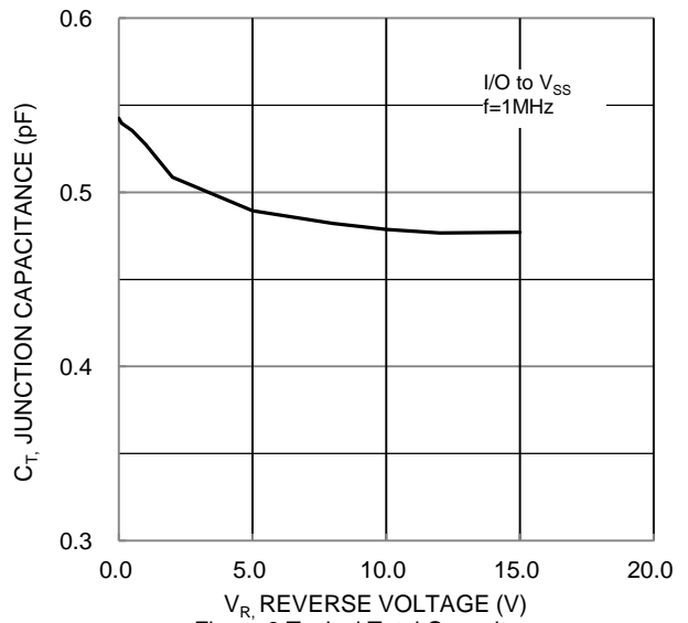
Figure 6 Typical Total Capacitance
