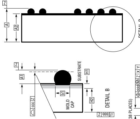
PACKAGE SIDE VIEW
