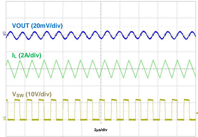
Figure 30. Output Voltage Ripple, IOOUT = 6A
