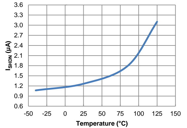
Figure 8. I_{SHDN} vs. Temperature
