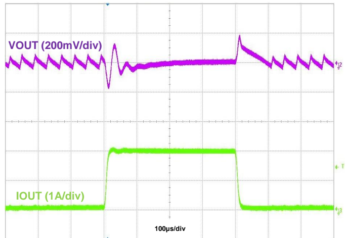
Figure 25. Load Transient, I_{OUT} = 50\text{mA} to 2\text{A} to 50\text{mA}
