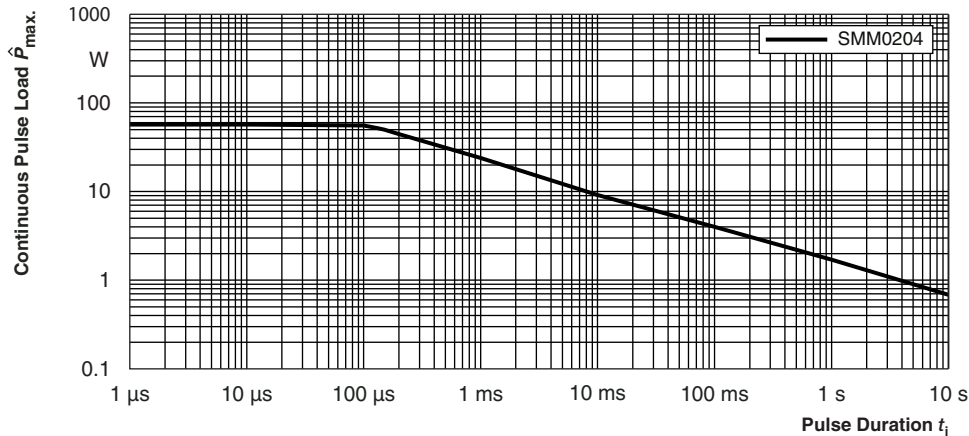
Maximum pulse load, continuous pulse; applicable if \bar{P} \leq P(\theta_{amb}) and \hat{U} \leq \hat{U}_{max,i} ; for permissible resistance change \pm (0.5\% R + 0.01 \Omega)
