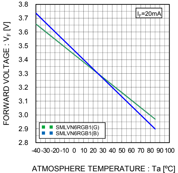
Fig.2-2 Forward Voltages - Atmosphere Temperature (G, B)
