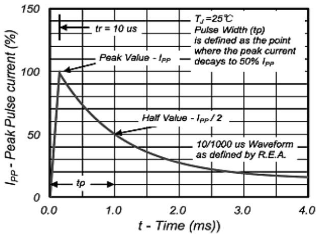
Fig 2: Pulse Waveform
