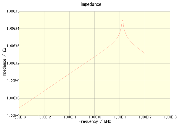
SLF10145T-470M1R4-PF
