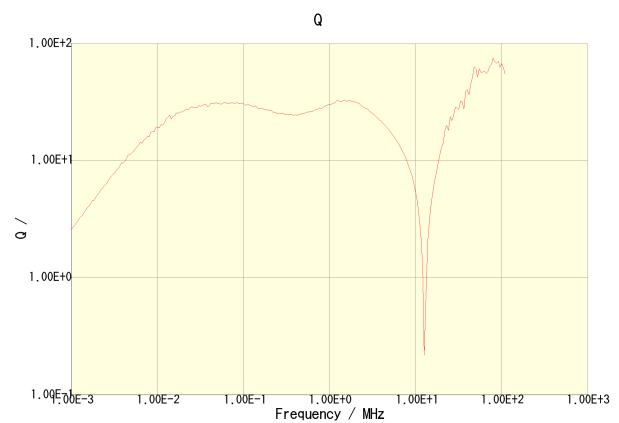
SLF10145T-470M1R4-PF
