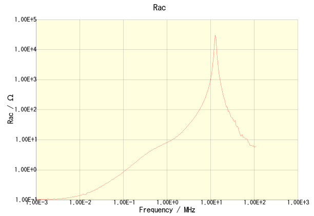
SLF10145T-470M1R4-PF
