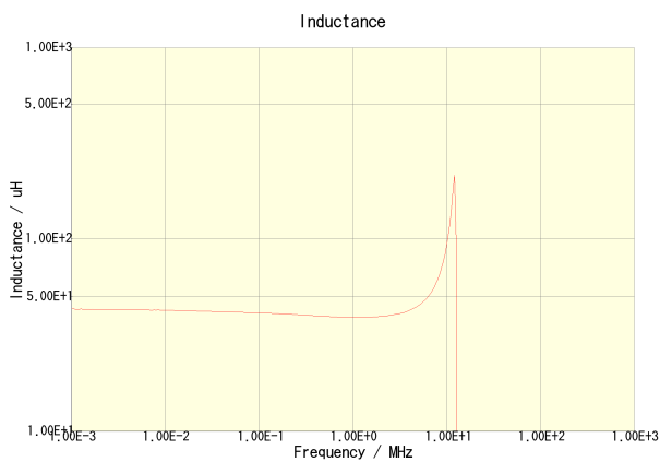
SLF10145T-470M1R4-PF
