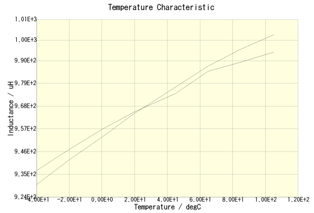
SLF10145T-102MR29-PF(DC = 0A) SLF10145T-102MR29-PF(DC = 0.145A)
