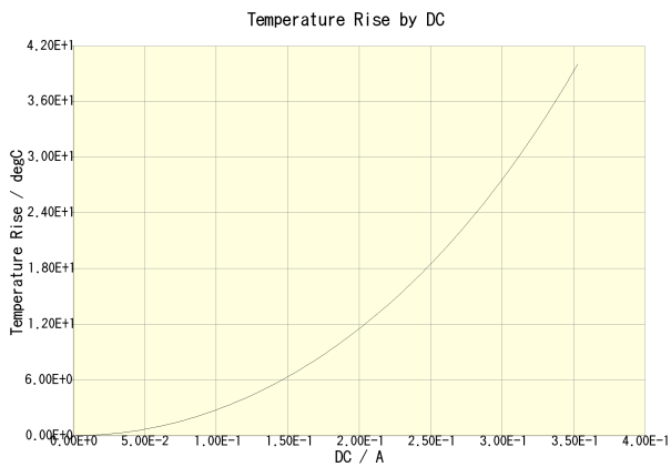
SLF10145T-102MR29-PF(Amb. Temp. = 20degc)
