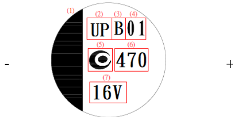
Figure 3 Marking
