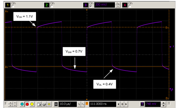
NanoDrive™ Output Waveform ( V_{OH} = 1.2\text{V} , V_{OL} = 0.4\text{V} , 10 pF Load; SiT1552AI-AI-D14-32.768)
