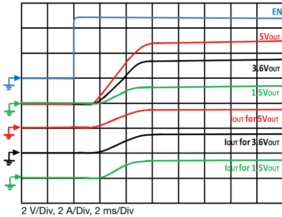
Fig. 21 - Typical Turn-on Delay, Rise Time C_{OUT} = 0.1 \mu\text{F} , C_{IN} = 4.7 \mu\text{F} , I_{OUT} = 1.5 \text{ A}
