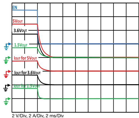
Fig. 26 - Typical Fall Time C_{OUT} = 200 \mu\text{F} , C_{IN} = 4.7 \mu\text{F} , I_{OUT} = 1.5 \text{ A}
