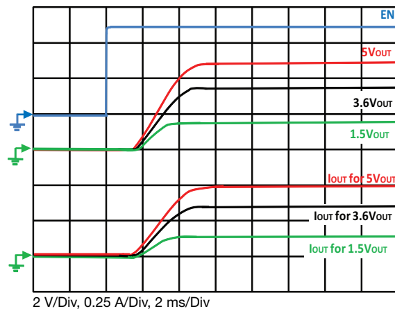
Fig. 22 - Typical Turn-on Delay, Rise Time C_{OUT} = 0.1 \mu\text{F} , C_{IN} = 4.7 \mu\text{F} , R_{OUT} = 10 \Omega
