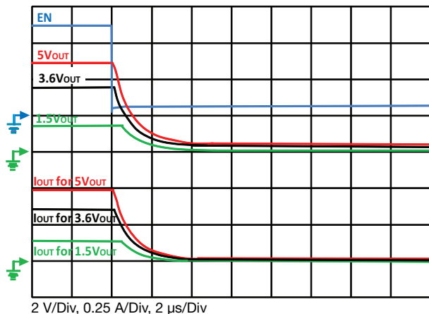
Fig. 25 - Typical Fall Time C_{OUT} = 0.1 \mu\text{F} , C_{IN} = 4.7 \mu\text{F} , R_{OUT} = 10 \Omega
