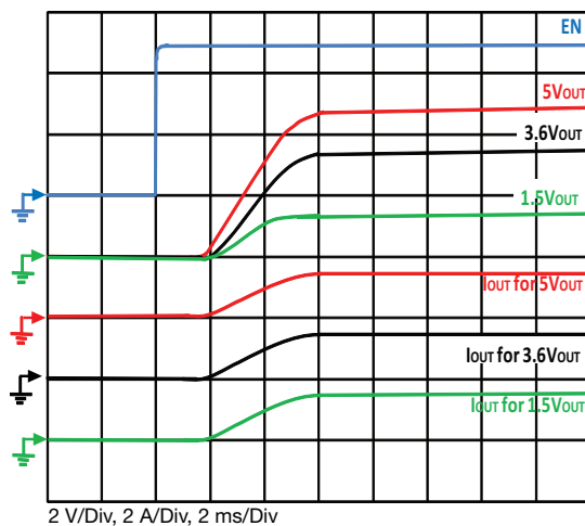
Fig. 23 - Typical Turn-on Delay, Rise Time C_{OUT} = 200 \mu\text{F} , C_{IN} = 4.7 \mu\text{F} , I_{OUT} = 1.5 \text{ A}
