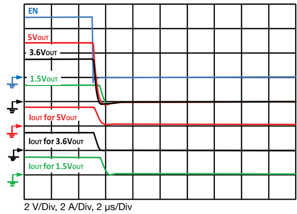
Fig. 24 - Typical Fall Time C_{OUT} = 0.1 \mu\text{F} , C_{IN} = 4.7 \mu\text{F} , I_{OUT} = 1.5 \text{ A}
