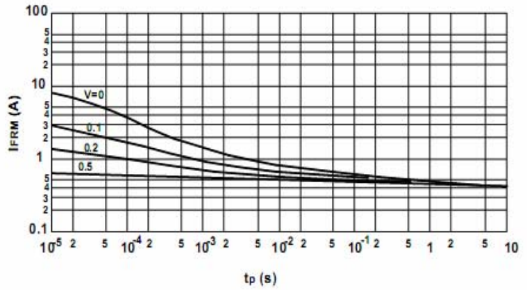
Admissible repetitive peak forward current vs. pulse duration
