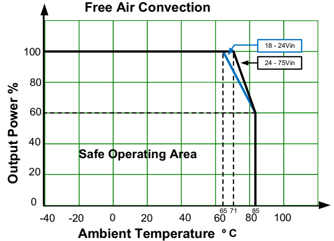
AM20EWM-4803SH50NZ, AM20EWM-4805SH50NZ
