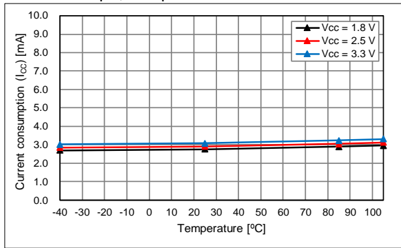
L CMOS = 5 pF, Temperature Characteristic
