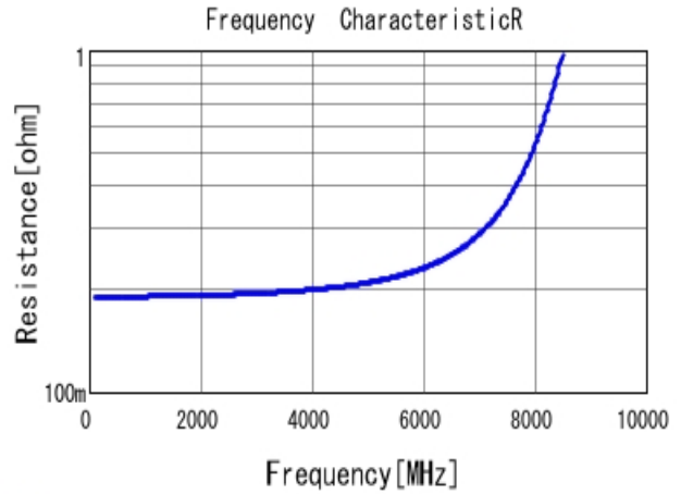
■ GQM1875C2E2R0BB12 R DCOV, 25degC
