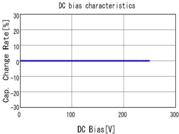
■ GQM1875C2E2R0BB12 C-DC bias capchange, 25.0degC, AC1V
