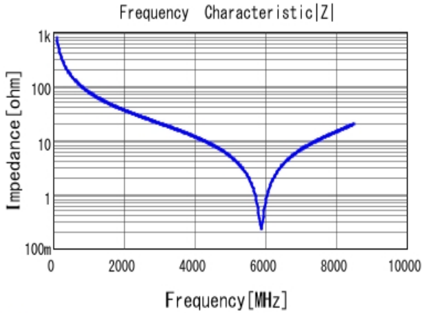
■ GQM1875C2E2R0BB12 |Z| DCOV, 25degC
