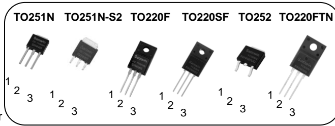
1. Gate 2. Drain 3. Source
