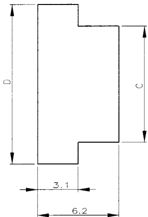
SECT. A-A
