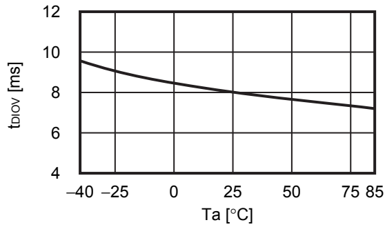
2. 9 t_{DI0V} vs. T_a
