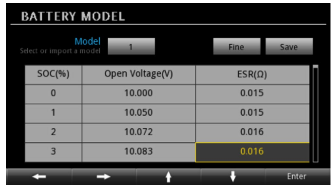
Figure 5. Battery model.
