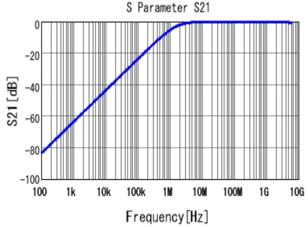
■ GCJ188R71H102KA01 S21 DC0V, 25degC
