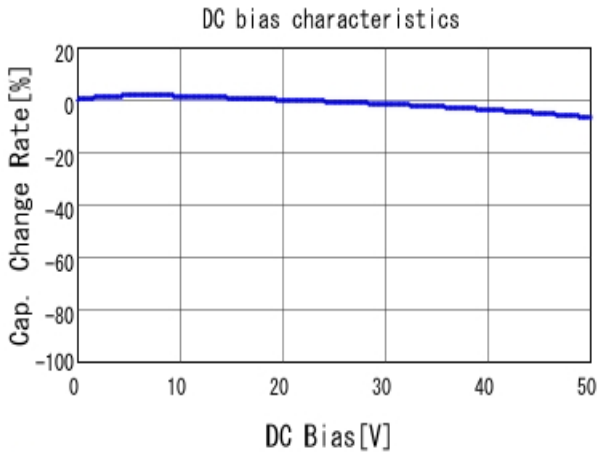
■ GCJ188R71H102KA01 C-DC bias capchange, 25.0degC, AC1.
