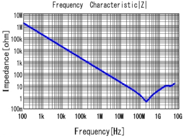
■ GCJ188R71H102KA01 |Z| DCOV, 25degC
