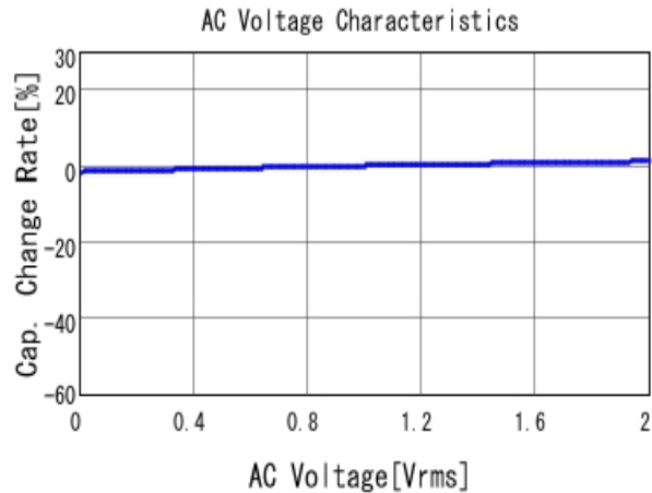
■ GCJ188R71H102KA01 C-AC Voltage capchange, DCOV, 25.0d
