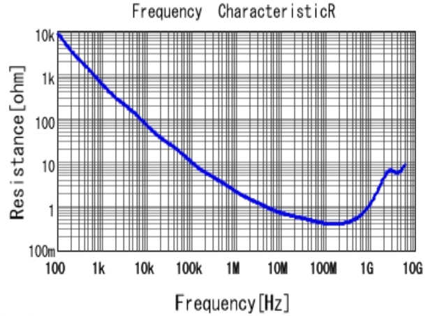
■ GCJ188R71H102KA01 R DCOV, 25degC
