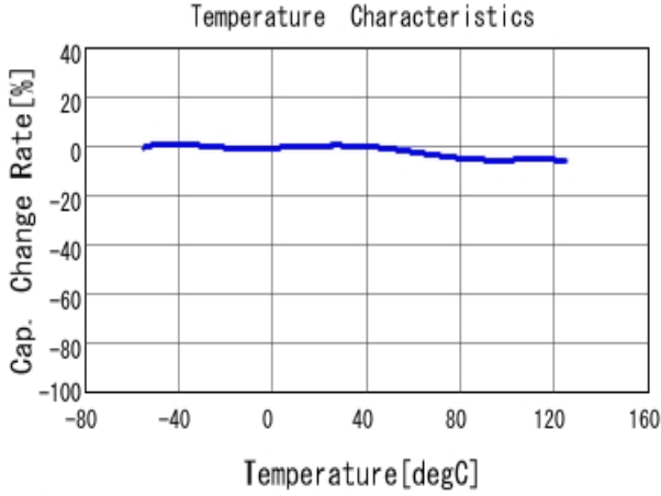
■ GCJ188R71H102KA01 C-Temp. capchange, DC0.0V, AC1.0V rm
