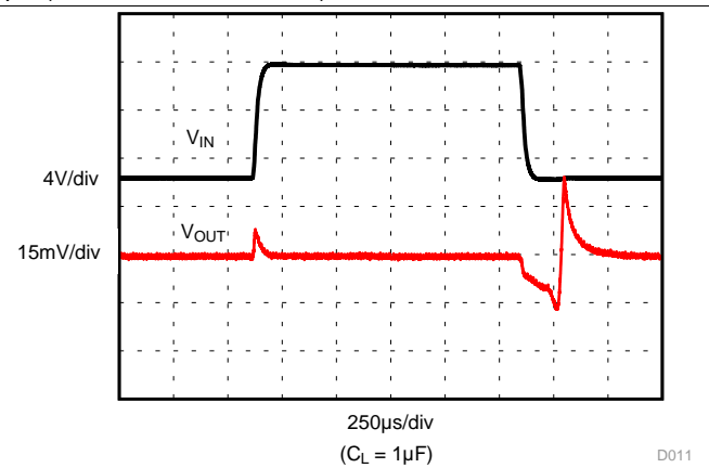
Figure 14. Line Transient
