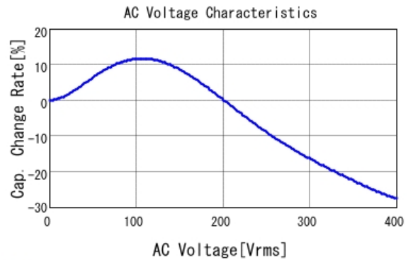
■ RDER73A223K3M1H03A C-AC Voltage capchange, DCOV, 25.0
