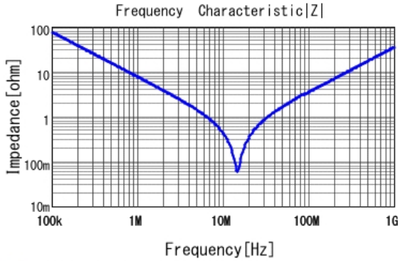
■ RDER73A223K3M1H03A |Z| DCOV, 25degC
