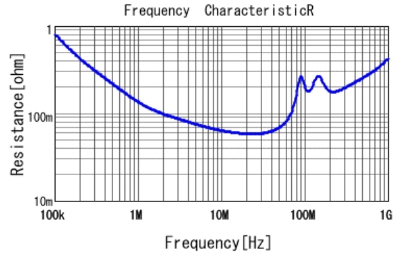
■ RDER73A223K3M1H03A R DCOV, 25degC
