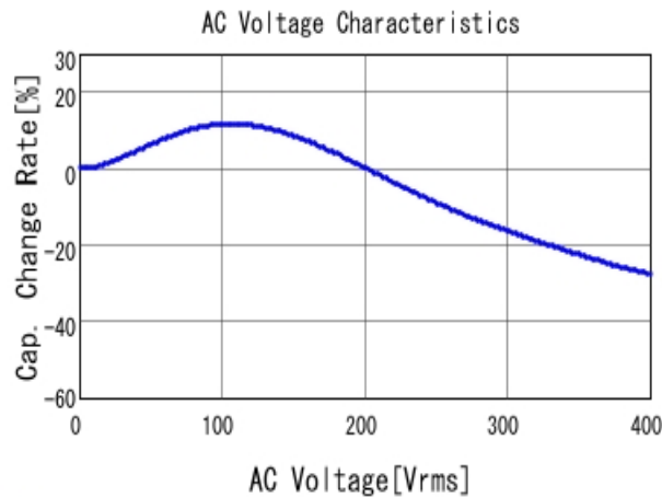
■ RDER73A223K3K1H03B C-AC Voltage capchange, DCOV, 25.0
