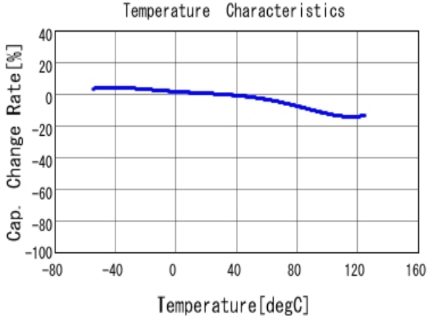
■ RDER73A223K3K1H03B C-Temp. capchange, DCOV, AC1Vrms
