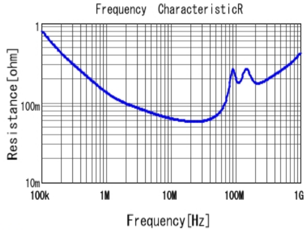
■ RDER73A223K3K1H03B R DCOV, 25degC
