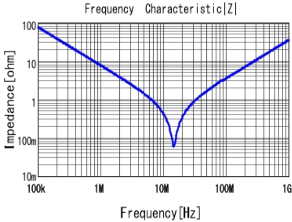
■ RDER73A223K3K1H03B |Z| DCOV, 25degC
