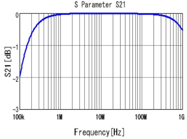
■ RDER73A223K3K1H03B S21 DCOV, 25degC
