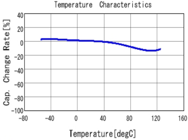
■ RDER72J333K3M1H03A C-Temp. capchange, DCOV, AC1Vrms
