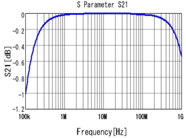
■ RDER72J333K3M1H03A S21 DCOV, 25degC
