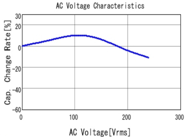
■ RDER72J333K3M1H03A C-AC Voltage capchange, DCOV, 25.0
