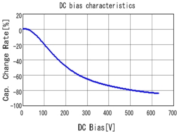
■ RDER72J333K3M1H03A C-DC bias capchange, 25.0degC, AC1
