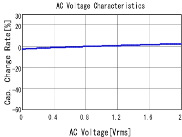
■ RDER72A105K2K1H03B C-AC Voltage capchange, DC0V, 25.0
