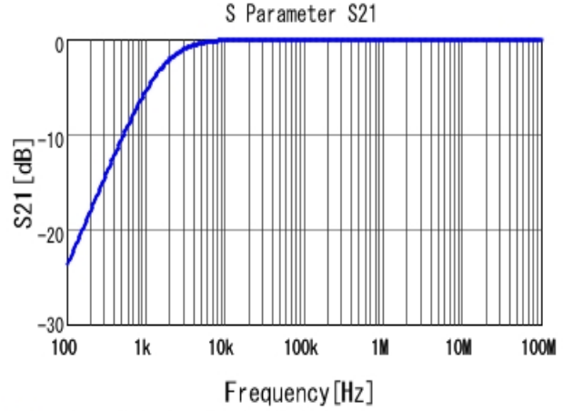
■ RDER72A105K2K1H03B S21 DC0V, 25degC
