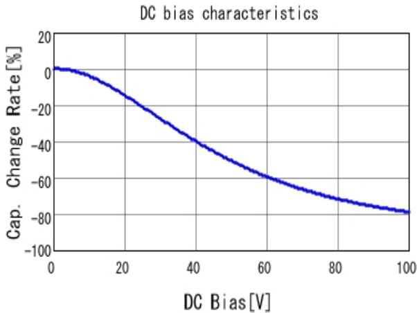
■ RDER72A105K2K1H03B C-DC bias capchange, 25.0degC, AC1
