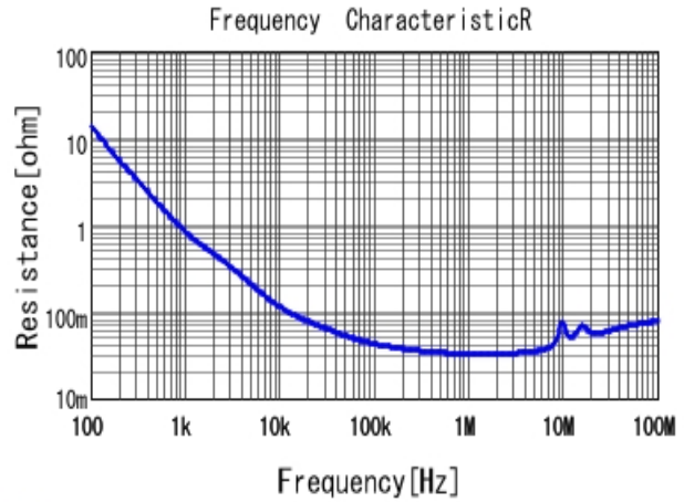
■ RDER72A105K2K1H03B R DC0V, 25degC
