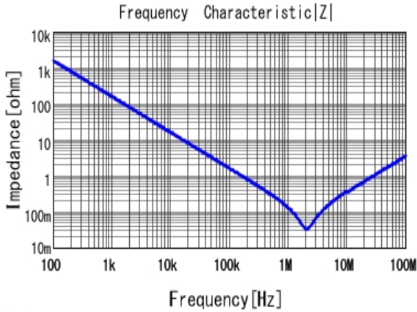
■ RDER72A105K2K1H03B |Z| DC0V, 25degC
