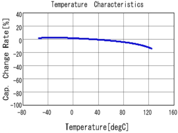
■ RDER72A105K2K1H03B C-Temp. capchange, DC0.0V, AC1.0Vr
