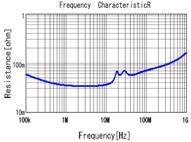
■ RDER71H474K1M1H03A R DC0V, 25degC
