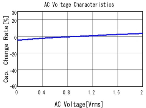
■ RDER71H474K1M1H03A C-AC Voltage capchange, DC0V, 25.0
