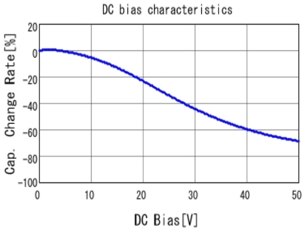
■ RDER71H474K1M1H03A C-DC bias capchange, 25.0degC, AC1
