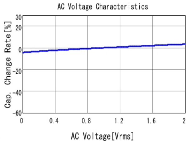
■ RDER71H225K2K1H03B C-AC Voltage capchange, DC0V, 25.0
