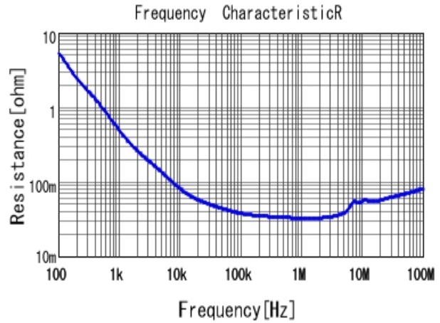
■ RDER71H225K2K1H03B R DC0V, 25degC
