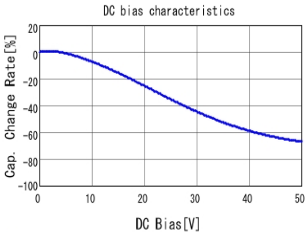
■ RDER71H225K2K1H03B C-DC bias capchange, 25.0degC, AC1
