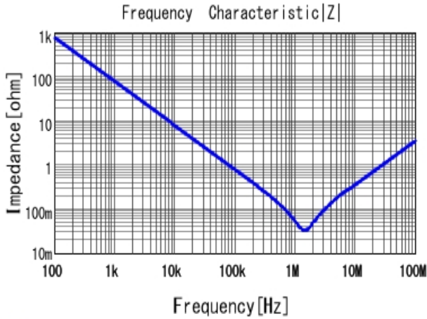
■ RDER71H225K2K1H03B |Z| DC0V, 25degC
