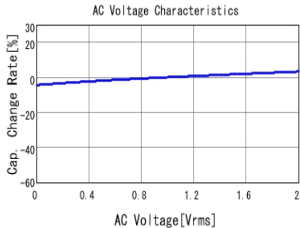
■ RDER71H105K2K1H03B C-AC Voltage capchange, DC0V, 25.0
