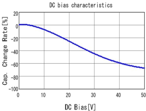
■ RDER71H105K2K1H03B C-DC bias capchange, 25.0degC, AC1
