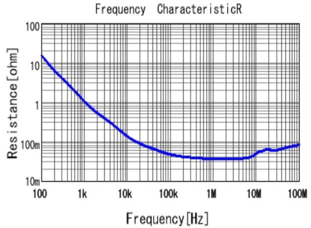
■ RDER71H105K2K1H03B R DC0V, 25degC
