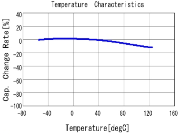
■ RDER71H105K2K1H03B C-Temp. capchange, DC0.0V, AC1.0Vr
