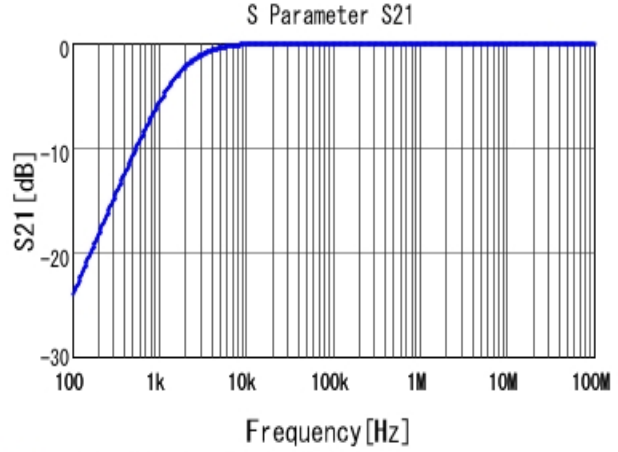
■ RDER71H105K2K1H03B S21 DC0V, 25degC
