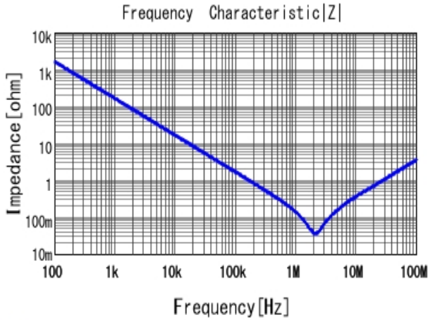
■ RDER71H105K2K1H03B |Z| DC0V, 25degC
