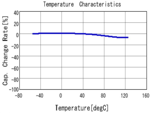
■ RDER71H104K0S1H03A C-Temp. capchange, DC0.0V, AC1.0Vr
