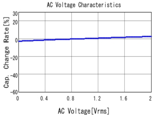
■ RDER71H104K0S1H03A C-AC Voltage capchange, DC0V, 25.0
