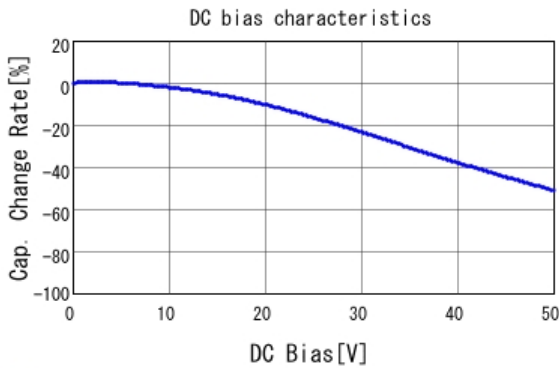
■ RDER71H104K0M1H03A C-DC bias capchange, 25.0degC, AC1
