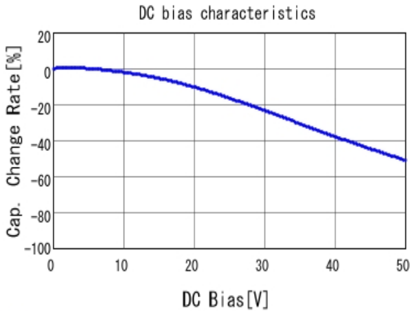
■ RDER71H104K0K1H03B C-DC bias capchange, 25.0degC, AC1
