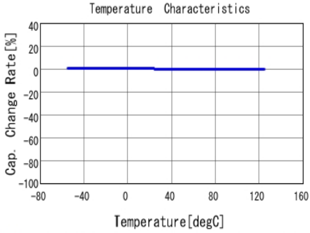
■ RDE5C1H330J0K1H03B C-Temp. capchange, DCOV, AC1Vrms
