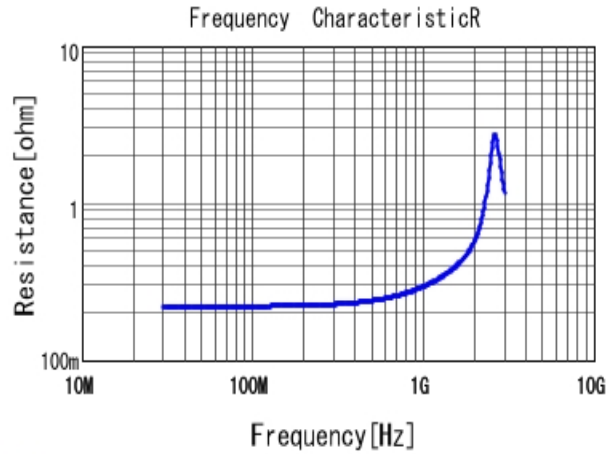
■ RDE5C1H330J0K1H03B R DC0V, 25degC
