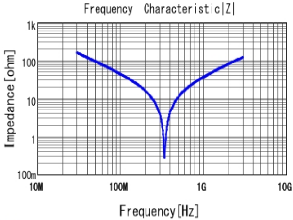
■ RDE5C1H330J0K1H03B |Z| DC0V, 25degC
