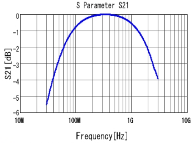
■ RDE5C1H330J0K1H03B S21 DCOV, 25degC
