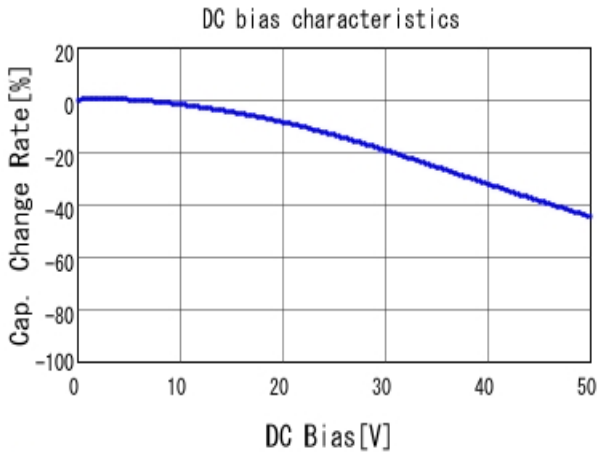
■ RCER71H224K1A2H03B C-DC bias capchange, 25.0degC, AC1
