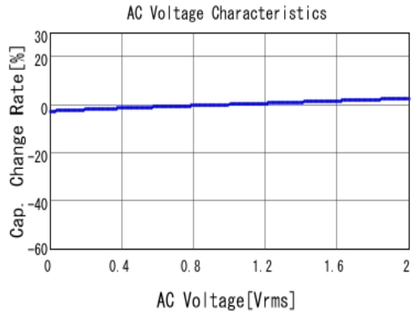
■ RCER71H224K1A2H03B C-AC Voltage capchange, DCOV, 25.0
