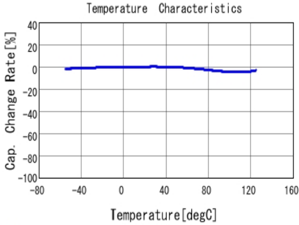
■ RCER71H224K1A2H03B C-Temp. capchange, DC0.0V, AC1.0Vr
