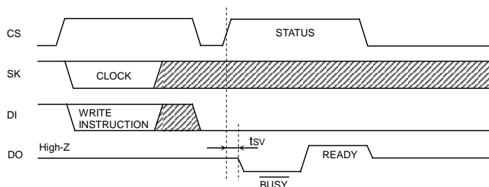
Figure 52. \overline{RD} status output timing chart
