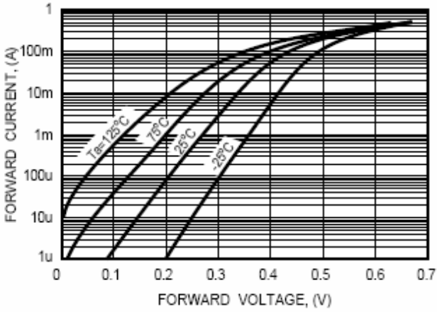
FIG. 1 - FORWARD CHARACTERISTICS
