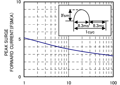
IFSM-CYCLE CHARACTERISTICS
