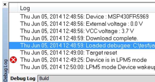
Figure 2-5. LPMx.5 Notifications
