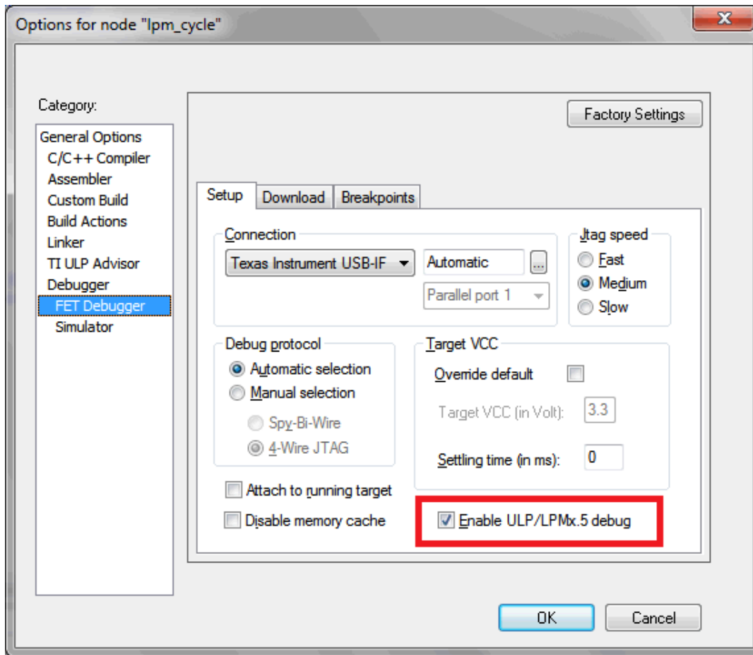
Figure 3-3. Debug Options
