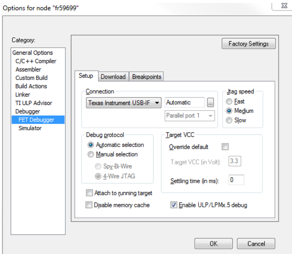
Figure 2-4. Enable Ultra-Low-Power Debug Mode
