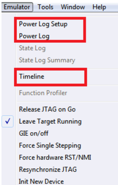
Figure 3-14. Emulator Pulldown Menu With EnergyTrace-Related Functions
