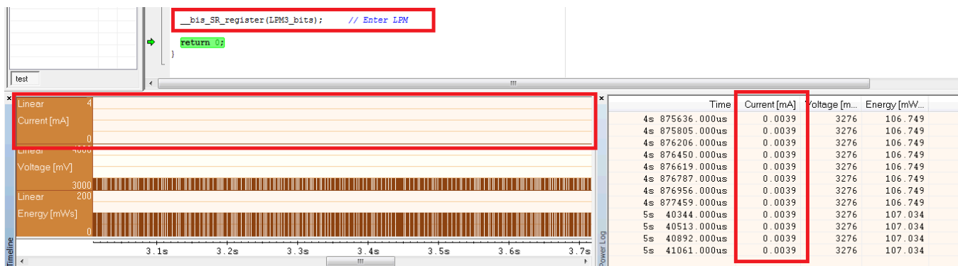
Figure 3-21. LPM3 Current When Executing with JTAG Signals Released
