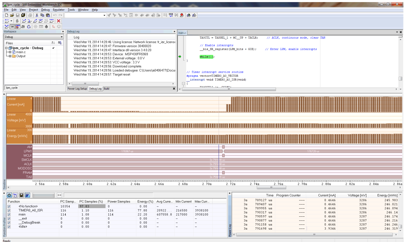
Figure 3-2. Debug Session With EnergyTrace++ Windows
