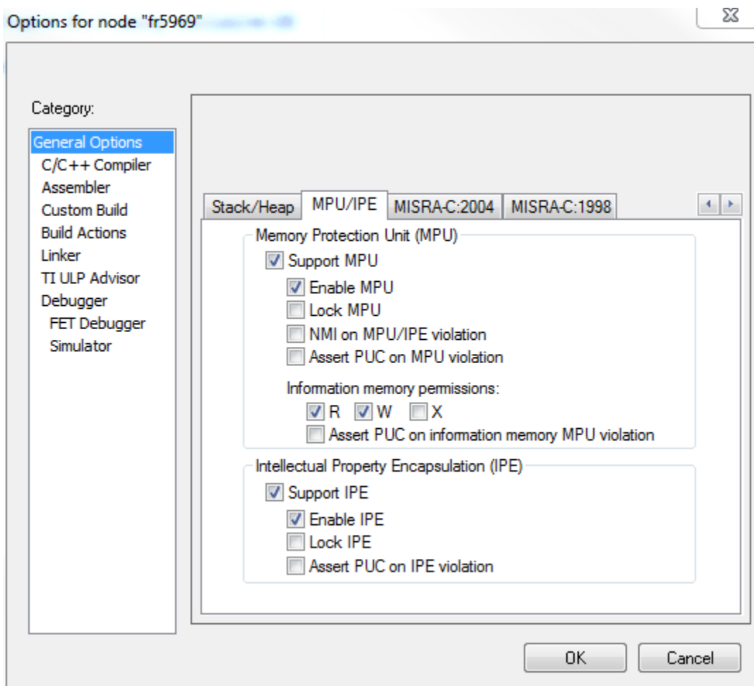
Figure 4-1. MPU Configuration Dialog
