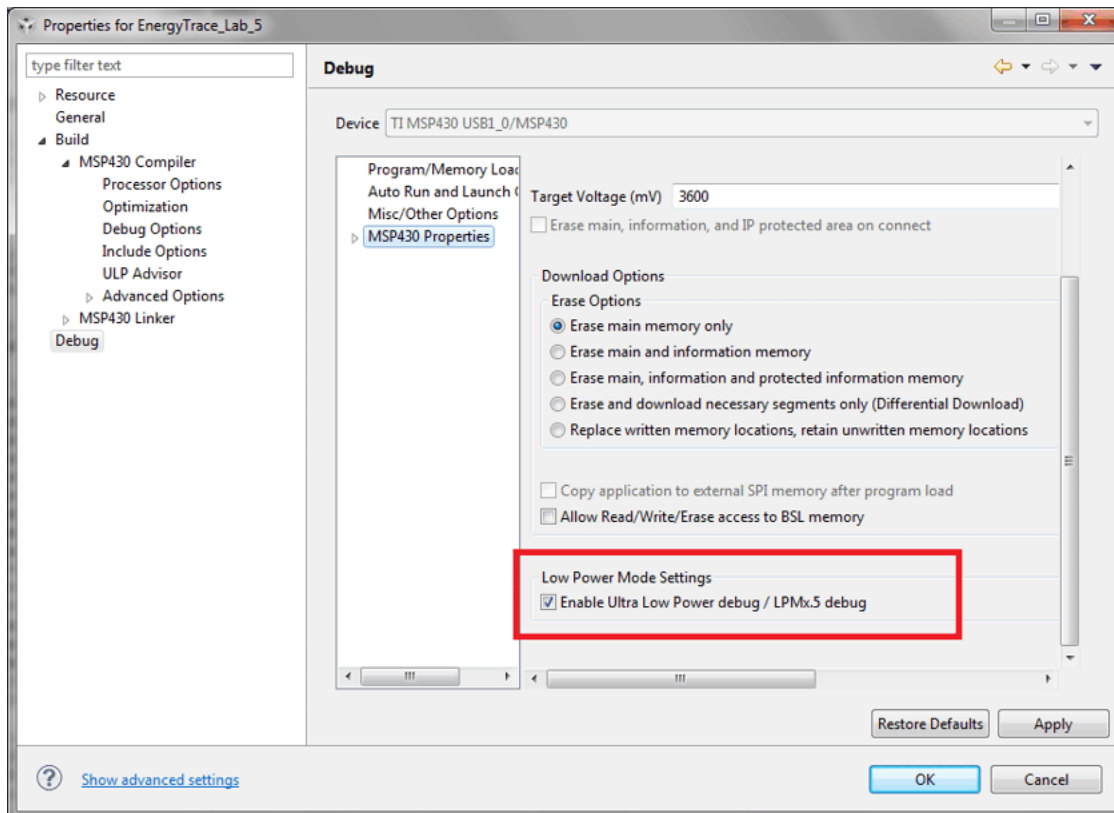
Figure 3-4. Debug Properties
