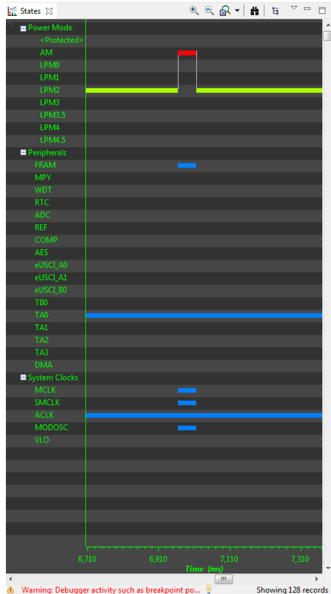
Figure 3-8. States Window
