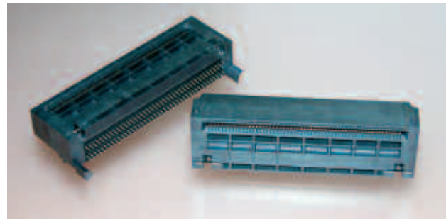
AdvancedMC Connector, Style B+ Part Number 1367703-X
