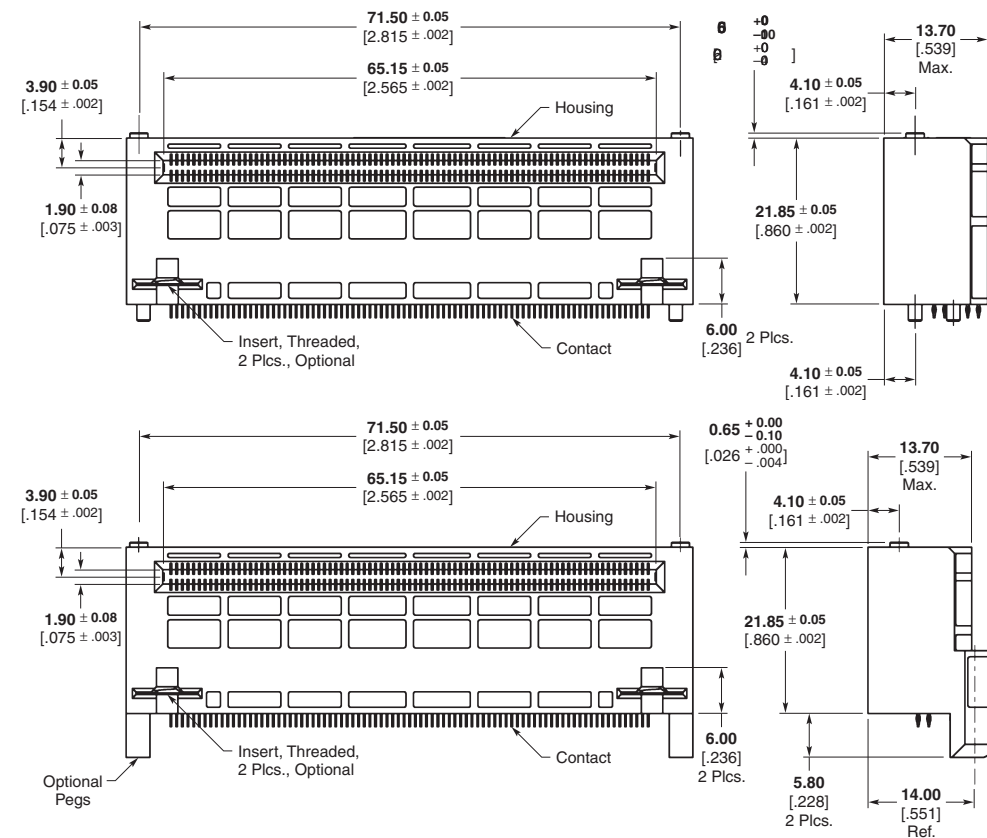
AdvancedMC Connector, Style B+ Part Number 1367703-X
