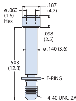
Kit Part Number 500-080-3 Kit Consists of 2 Jackscrews and 2 E-Rings
