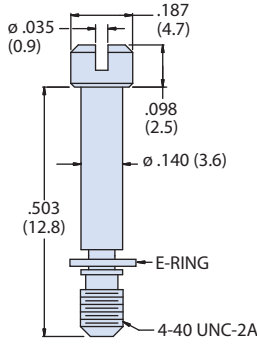
Kit Part Number 500-081-3 Kit Consists of 2 Jackscrews and 2 E-Rings
