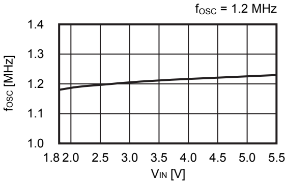
(3) Oscillation frequency (f osc ) vs. Input voltage (V IN )
