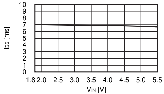
(5) Soft-start time (t SS ) vs. Input voltage (V IN )
