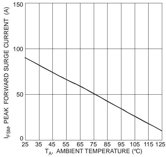
Fig. 8 Non-Repetitive Forward Surge Current Derating Curve
