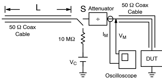
Figure 15. Simplified Schematic of a Typical TLP System
